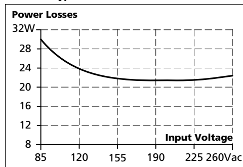
Fig. 9-4 Losses vs. input voltage at 48V, 5A, typ.
