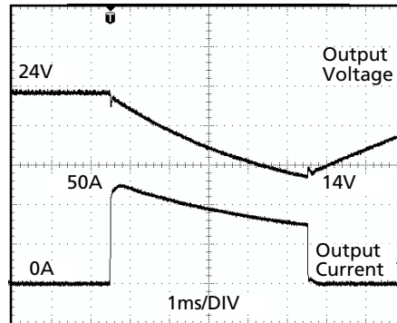
Peak load 50A (resistive) for 5ms Output voltage dips from 24V to 14V.
