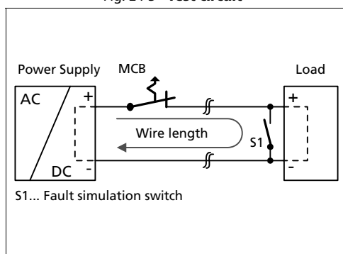
Fig. 24-3 Test circuit
