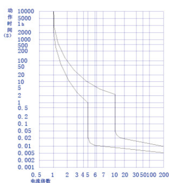
C Curve
