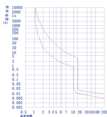
D Curve
